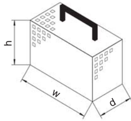
Type A Governor hood for Ø200 pulley, suitable for BODE-controller w=250, h=230, d=100-175 art. no. 78627 governor hood type A
