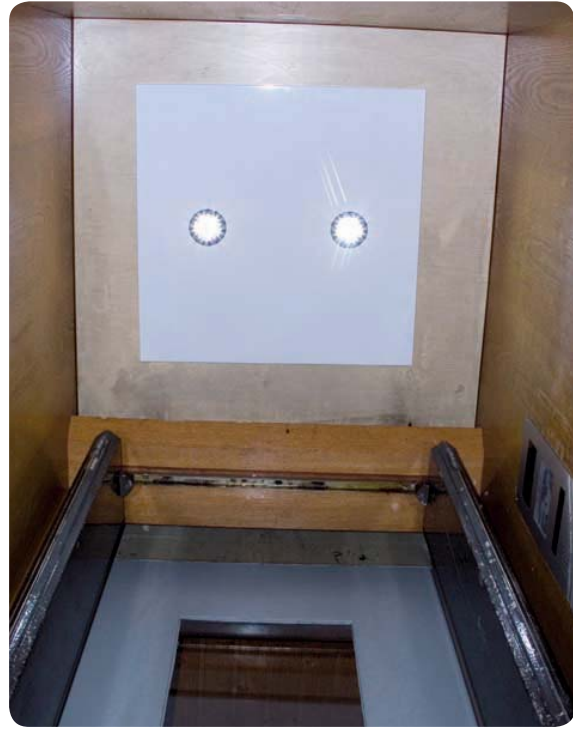
Mounting example: Retrofitting of a white aluminium ceiling in an old wooden cabin
