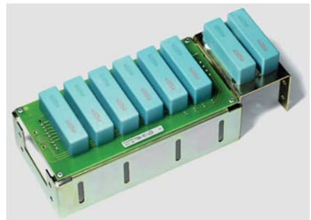
MB 6 With printed circuit board plug-in connection
